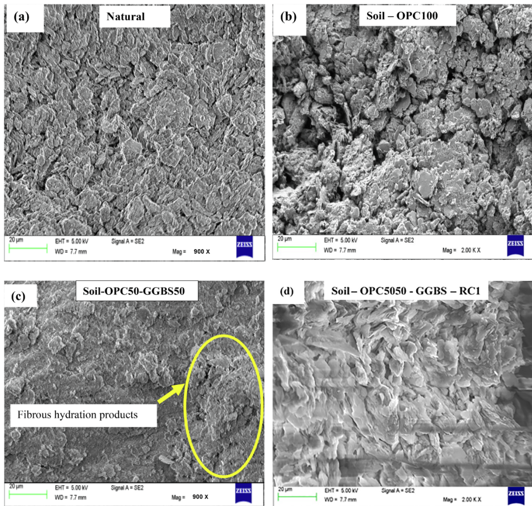
Fig. 16. Micrographs of stabilized soils (a) Natural soil, (b) SEM of OPC-stabilized soil, (c) SEM of OPC-GGBS-stabilized soil, (d) SEM of OPC-GGBS-RC-stabilized soil.
