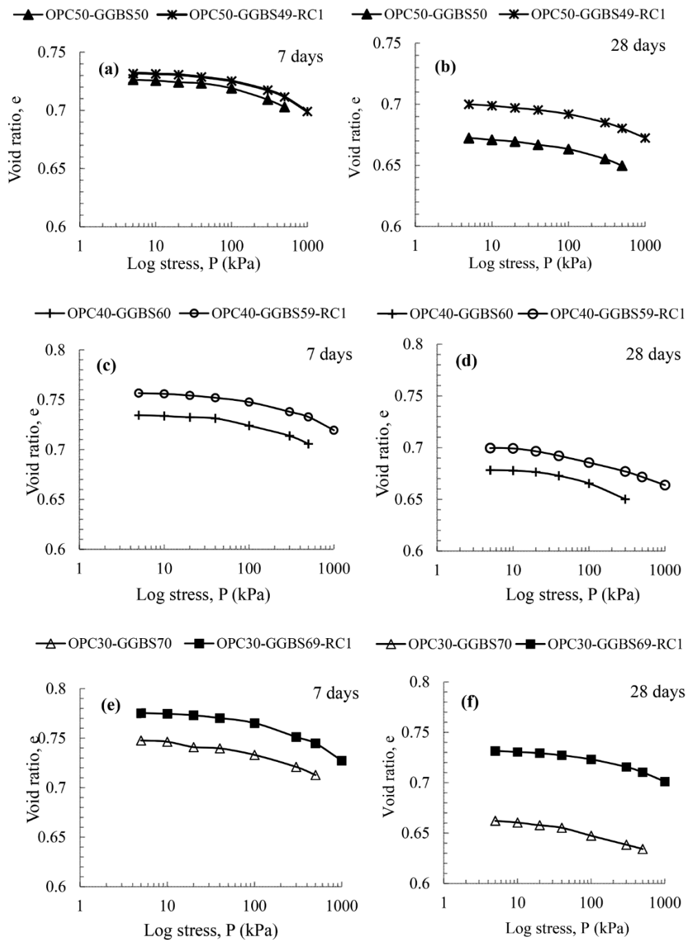
Fig. 8. Stabilized soil e vs. log P consolidation curve showing effect of RC (a) 7-day cured stabilized soil for 50% OPC replacement, (b) 28-day cured stabilized soil for 50% OPC replacement, (c) 7-day cured stabilized soil for 60% OPC replacement, (d) 28-day cured stabilized soil for 60% OPC replacement, (e) 7-day cured stabilized soil 70% OPC replacement, (f) 28-day cured stabilized soil for 70% OPC replacement.
