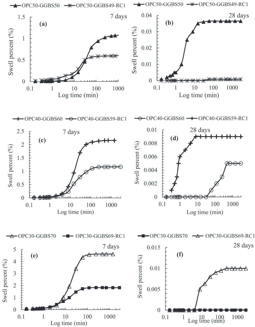
Fig. 4. Stabilized soil swelling showing effect of RC (a) 7-day cured stabilized soil for 50% OPC replacement, (b) 28-day cured stabilized soil for 50% OPC replacement, (c) 7-day cured stabilized soil for 60% OPC replacement, (d) 28-day cured stabilized soil for 60% OPC replacement, (e) 7-day cured stabilized soil for 70% OPC replacement (f) 28-day cured stabilized soil for 70% OPC replacement.
