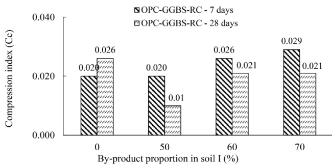
Fig. 7. Stabilized soil compression indices of 7- & 28-day cured stabilized soil for 50, 60 & 70% OPC replacement.
