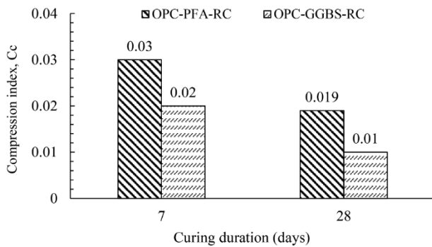
Fig. 11. Comparing between compression indices of 7- & 28-day cured stabilized soil composed of PFA and GGBS.
