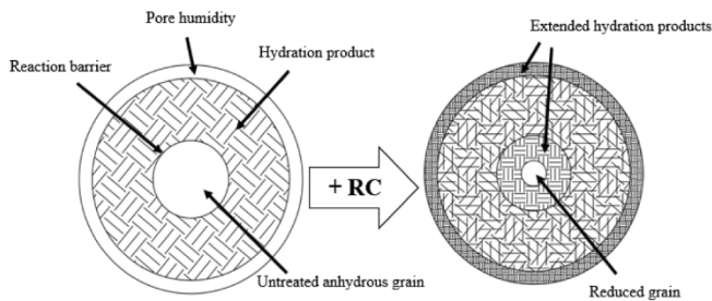
Fig. 15. Description of mechanism of stabilization with the inclusion of RC.
