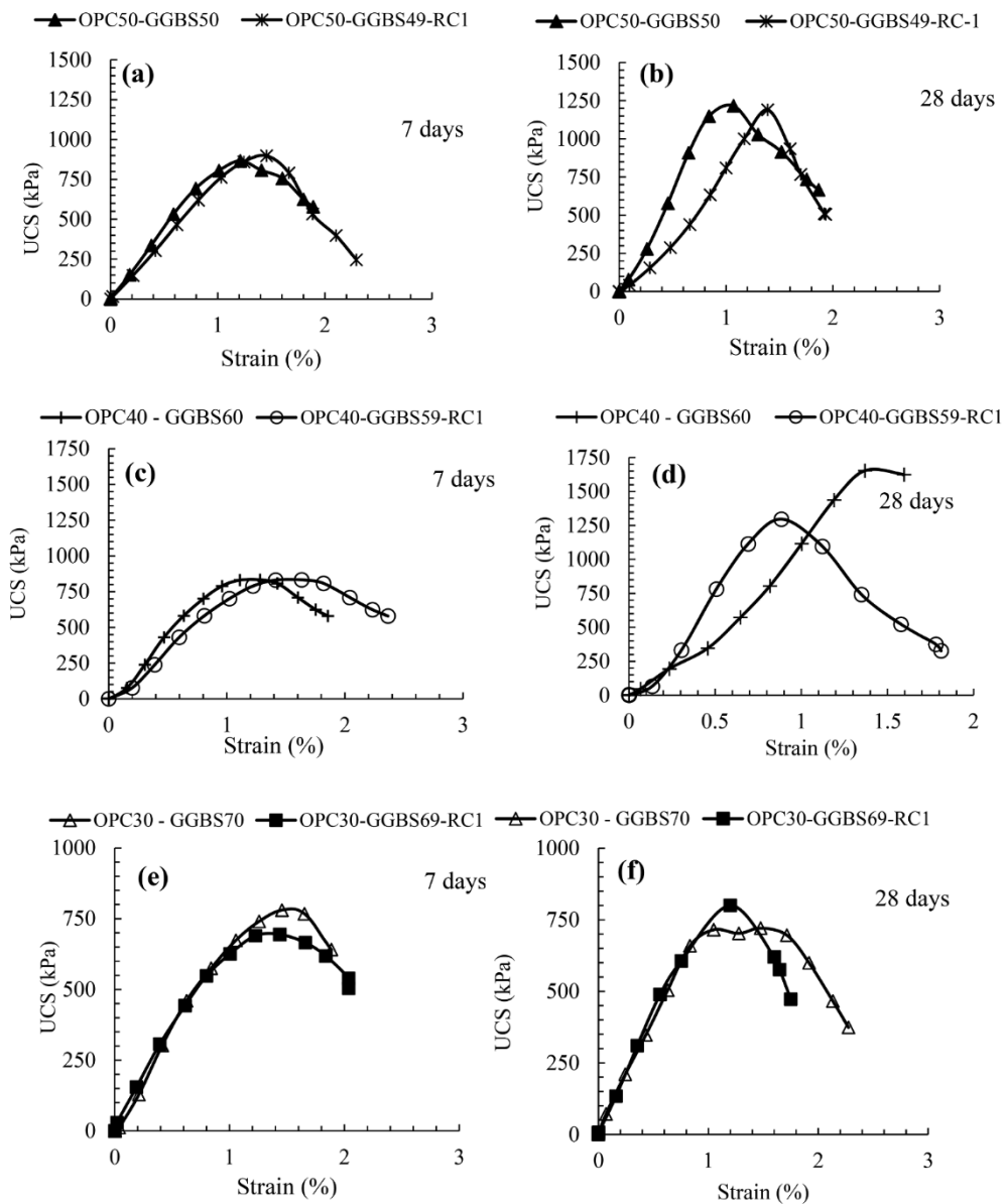
Fig. 13. Unconfined compressive strength of stabilized soil indicating the effect of RC (a) 7-day cured stabilized soil for 50% OPC replacement, (b) 28-day cured stabilized soil for 50% OPC replacement, (c) 7-day cured stabilized soil for 60% OPC replacement, (d) 28-day cured stabilized soil with and without RC for 60% OPC replacement, (e) 7-day cured stabilized soil for 70% OPC replacement, (f) 28-day cured stabilized soil for 70% OPC replacement.
