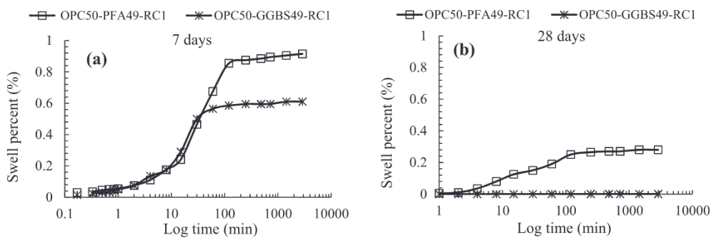
Fig. 5. Swell potential of stabilized soil (a) comparing between 7-day cured RC-modified soil composed of PFA and GGBS, (b) comparing between 28-day cured RC-modified soil composed of PFA and GGBS.
