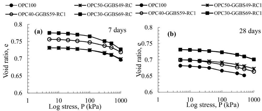
Fig. 6. Stabilized soil consolidation (a) e vs. log P curve of 7-day cured stabilized soil for 50, 60 & 70% OPC replacement, (b) e vs. log P curve of 28-day cured stabilized soil for 50, 60 & 70% OPC replacement.
