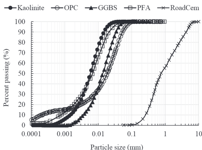
Fig. 2. Analysis of particle size of soil and binders.
