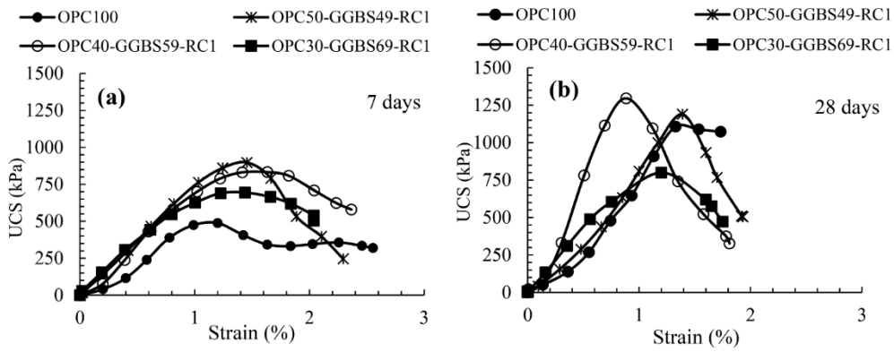
Fig. 12. Unconfined compressive strength of stabilized soil (a) 7-day cured stabilized soil for 50, 60 & 70% OPC replacement, (b) 28-day cured stabilized soil for 50, 60, 70% OPC replacement.
