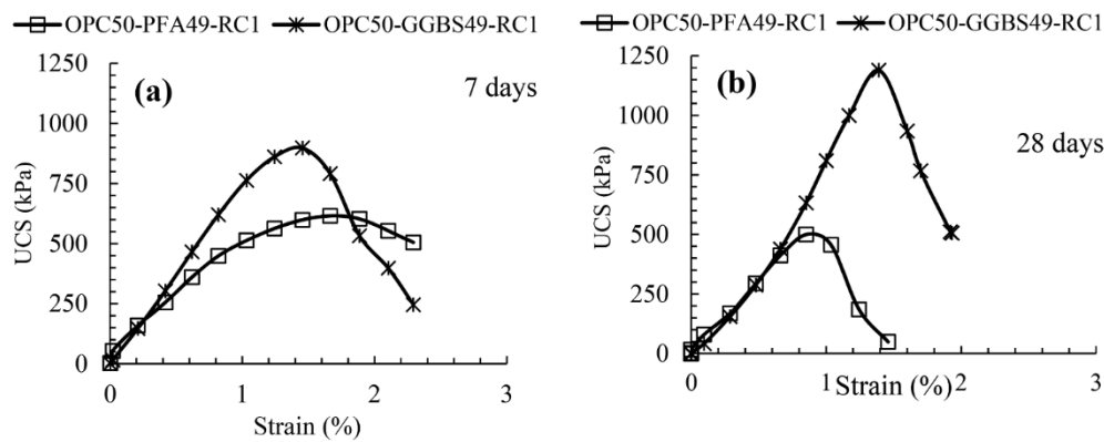
Fig. 14. Stabilized soil unconfined compressive strength (a) comparing between 7-day cured RC-modified soil composed of PFA and GGBS, (b) comparing between 28-day cured RC-modified soil composed of PFA and GGBS.
