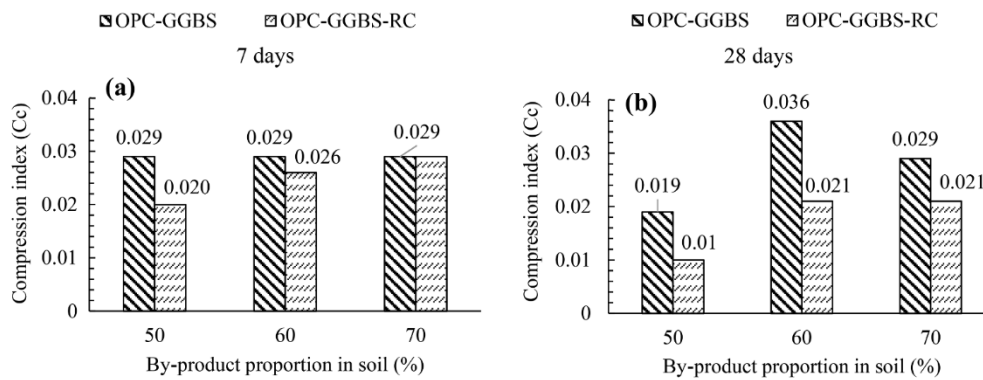
Fig. 9. Stabilized soil compression index showing effect of RC (a) 7-day cured stabilized soil for 50, 60 & 70% OPC replacement, (b) 28-day cured stabilized soil for 50, 60 & 70% OPC replacement.
