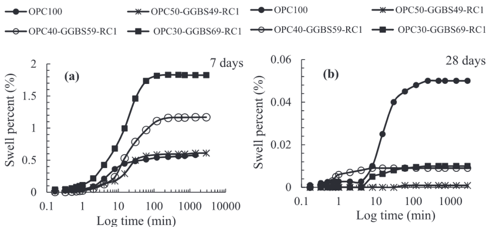
Fig. 3. Swell potential of stabilized soil (a) 7-day cured stabilized soil for 50, 60 & 70% OPC replacement, (b) 28-day cured stabilized soil for 50, 60, 70% OPC replacement.
